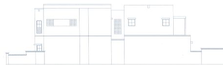
Lot Side Elevation
